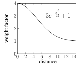
Figure 2: Weight update function for an edge e at x hops from the “problem” node n .
