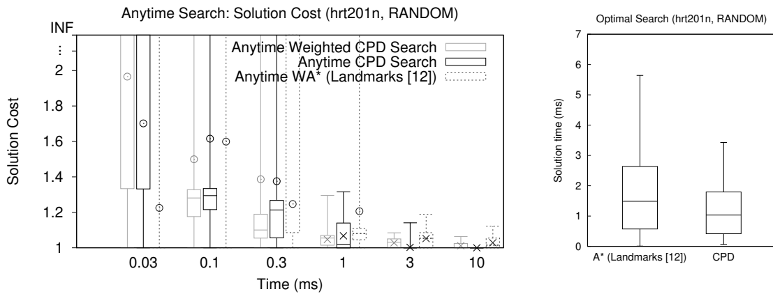
Figure 4: Anytime and Optimal Search with RANDOM perturbations. (Left) We show the distribution of best solution costs (normalised by optimal cost) at different time cutoffs. A cross on each box-plot indicates average (normalised) solution cost (where defined). When the max is infinite a circle represents the largest non-infinity normalised solution cost. (Right) We report (CPU) time distributions for optimal search on hrt201n.
